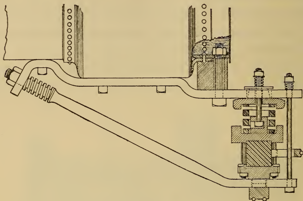
FIG. 42.—SPRING MOUNTING.
